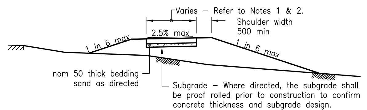
TYPICAL SECTION (Where no kerb & channel exist)
