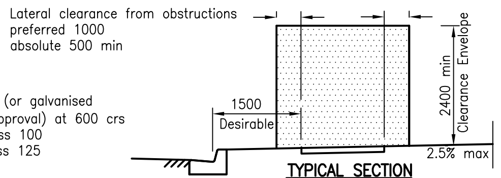
TYPICAL SECTION (Where no kerb & channel exist)
