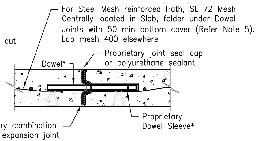
DETAIL 'A' PREFORMED KEY JOINT WITH DOWEL * Dowel maybe eliminated for mass concrete paths
