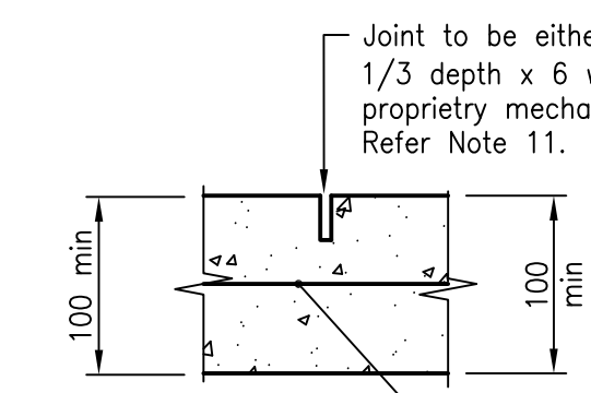
CONTROL JOINT (CJ) Shown C.J. on plans
