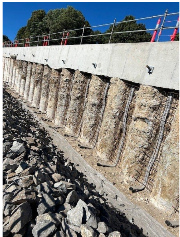
Retaining wall
